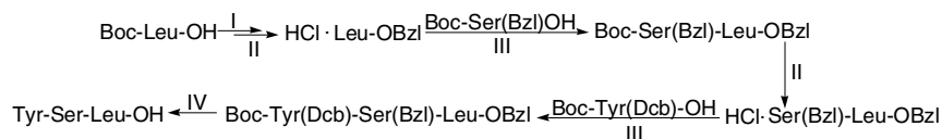
Scheme 1. Synthetic route of YSL with normal protective strategy. Reagents: (I) CsCO 3 , C 6 H 5 CH 2 Br; (II) HCl/CH 3 CO 2 C 2 H 5 (6 mol/L); (III) DCC/HOBt/NMM with corresponding carboxyl component; (IV) HF.
