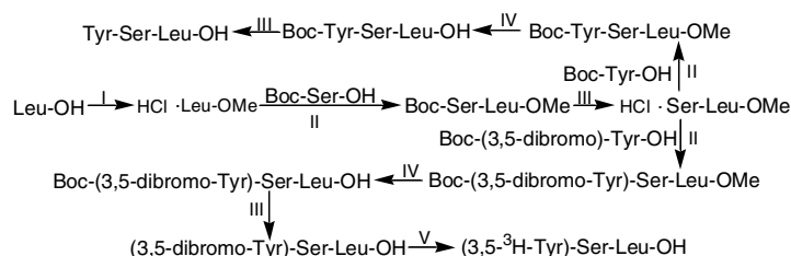
Scheme 2. Synthetic route of YSL with minimal protective strategy. Reagents: (I) HCl/CH 3 OH; (II) DCC/HOBt/NMM with corresponding carboxyl component; (III) HCl/CH 3 CO 2 C 2 H 5 (6 mol/L); (IV) NaOH/H 2 O/CH 3 OH; (V) 3 H 2 and 10% Pd/C.
